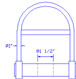
HEAVY DUTY SWIVEL-HINGE TYPE BAIL
